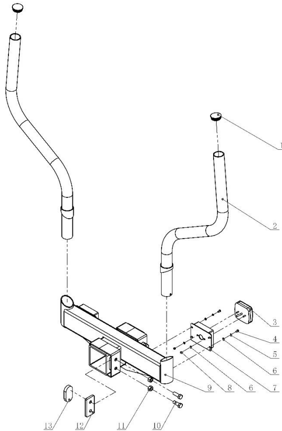
Back-end frame Components
