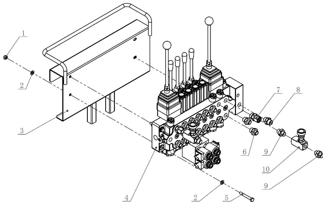
Multi-way valve assembly
